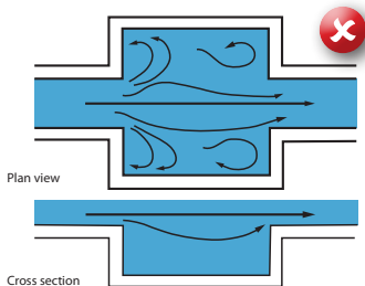
Poor design, the silt passes through
