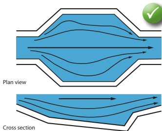
Good design with gradual changes of cross section
