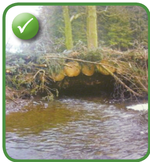
Good practice log bridge
